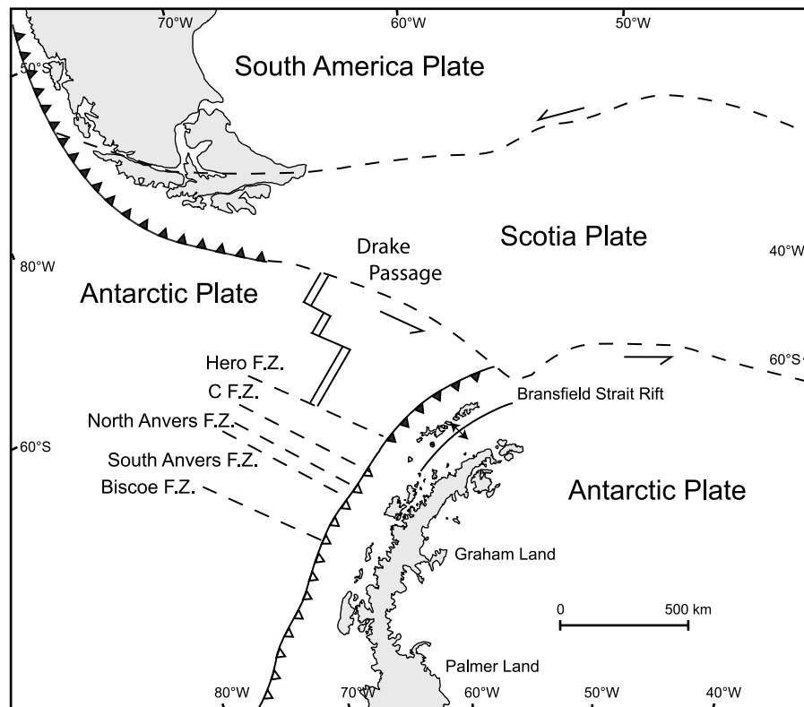
Figure 1. Plate tectonic map of the Antarctic Peninsula and Scotia Arc region. Map symbols are as follows: black sawtooth patterns are currently active subduction zones, white sawtooth patterns are currently inactive subduction zones, white rectangles are currently inactive spreading ridges, and dashed lines are fracture zones (arrows represent motion on transform plate boundaries).
