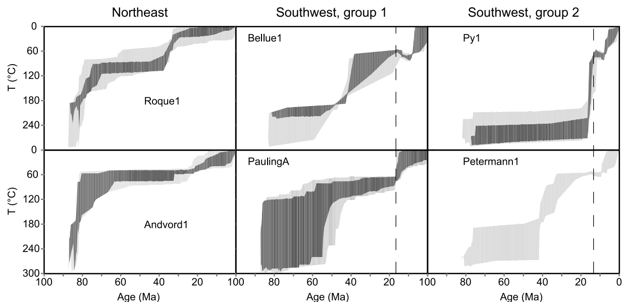
Figure 7. Results from HeFTy inverse models. Plots are arranged into groups in a fashion similar to Figure 3 and depict the cumulative envelopes for all samples in each geographic location. Opacity of the envelopes is based upon the goodness of fit (GOF), with GOF > 0.05 in light gray and GOF > 0.5 in dark gray. See Ketcham [2005] and the auxiliary material for details on HeFTy statistical methods.
